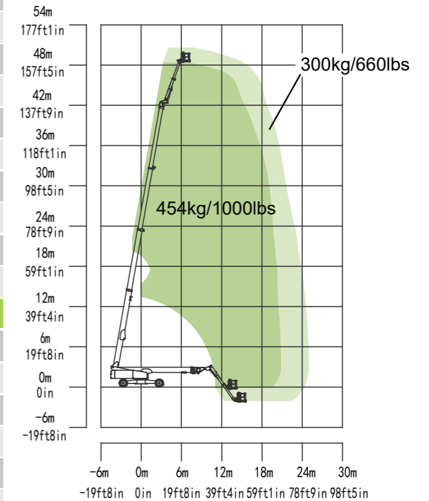
Range of Motion ZT51JEH-V
